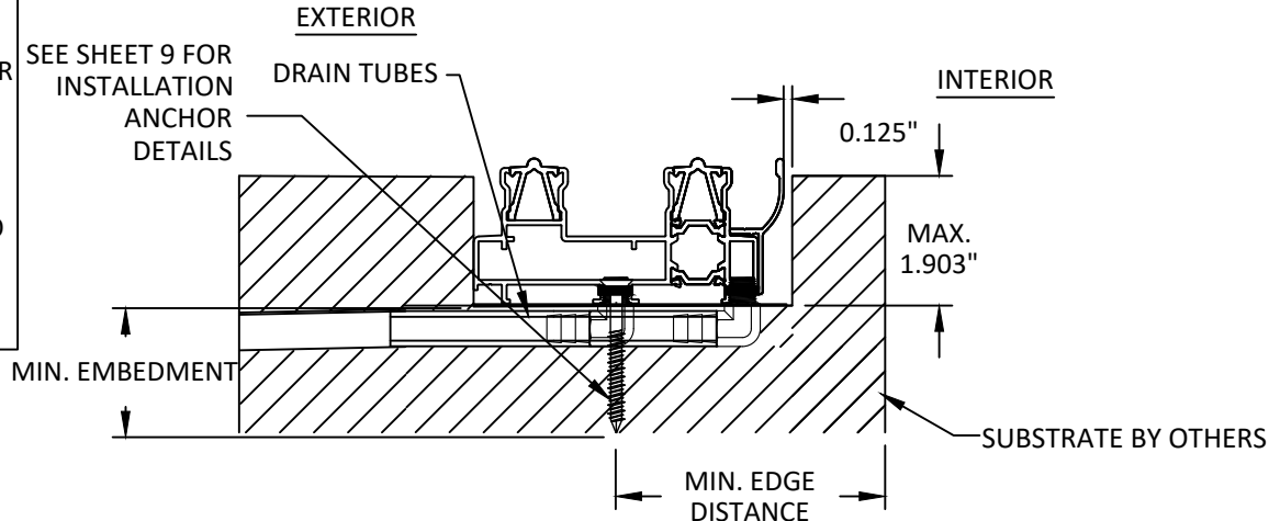
D 8 ANCHOR DETAIL THROUGH FRAME INSTALLATION (SILL) OPTIONAL SUNKEN 2-TRACK INSTALLATION
