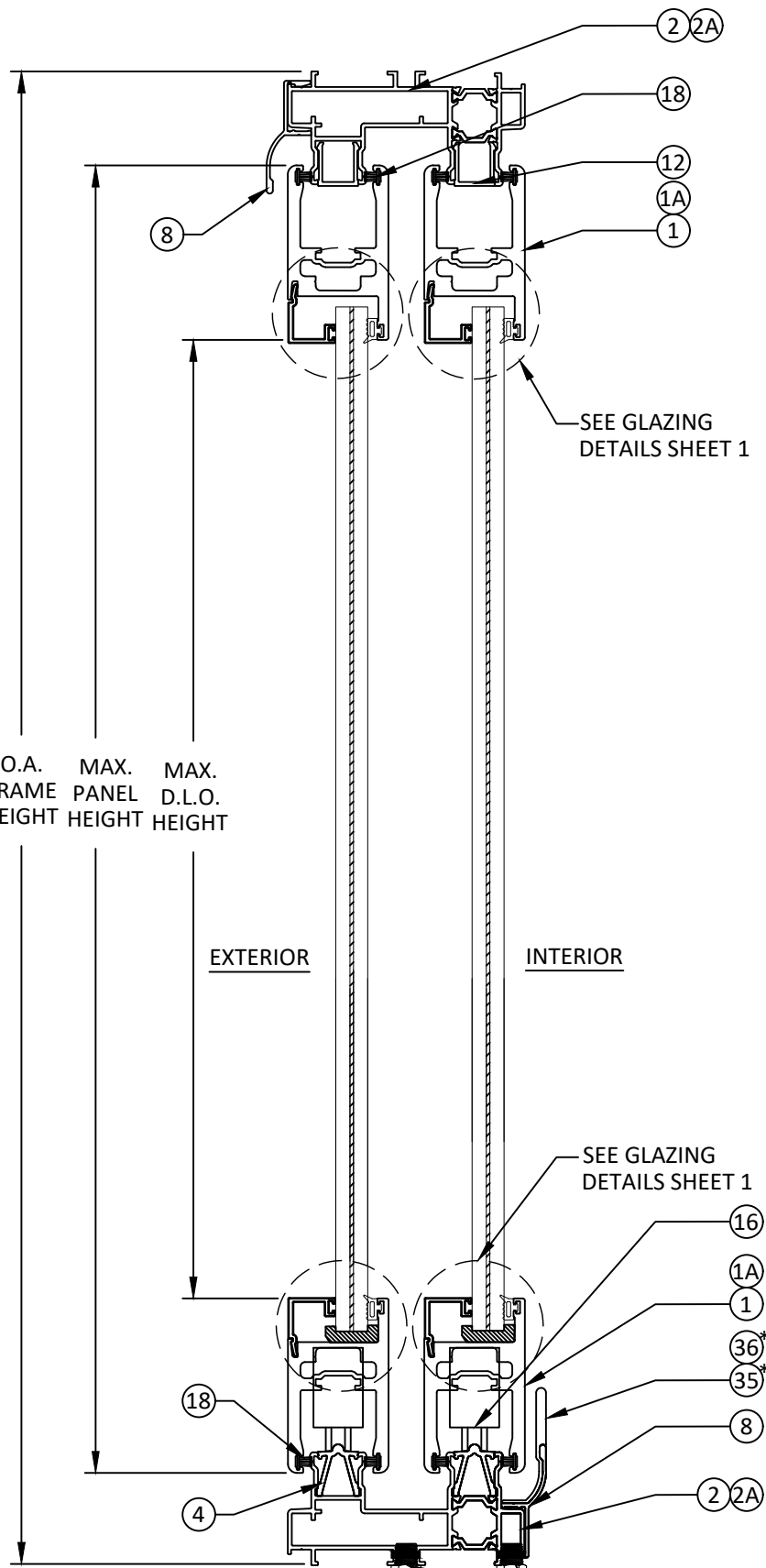
VERTICAL SECTION SLIDING GLASS DOOR OPTIONAL SUNKEN SILL 2 TRACKS SHOWN, 3 TRACKS QUALIFIED
